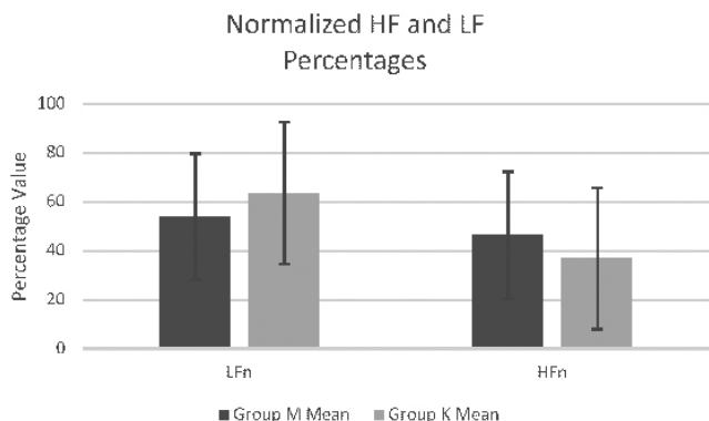
Figure 1. Mean values of HFnu and LFn, and standard deviation values in the group HFnu: Normalized high frequency, LFn: normalized low frequency
